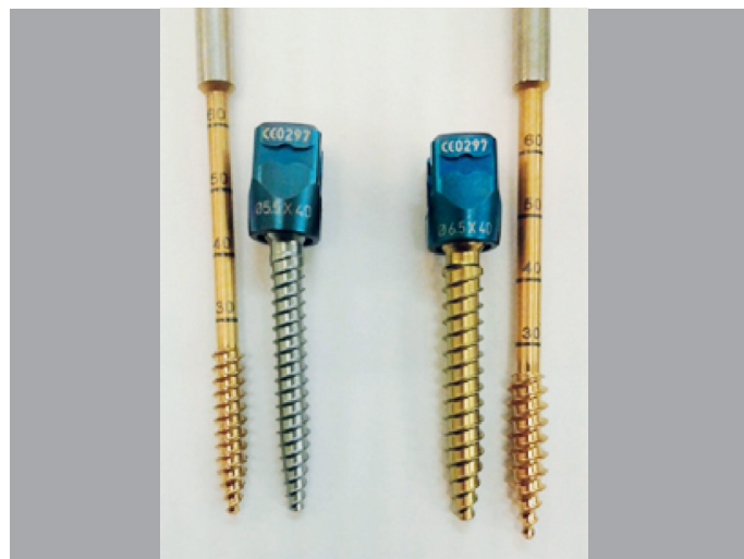
Figure 1. Photograph of the screws and respective taps used in the study - on the left, the tap and the 5.5 mm screw and, on the right, the tap, and the 6.5 mm screw (Globus). Screw characteristics – 5.5 mm screw: screw core 4.5 mm, between threads 1.8 mm; 6.5 mm screw: screw core 5.0 mm, between threads 2.1 mm. 6.5 mm, 5.5 mm, and 4.5 mm taps were used.
