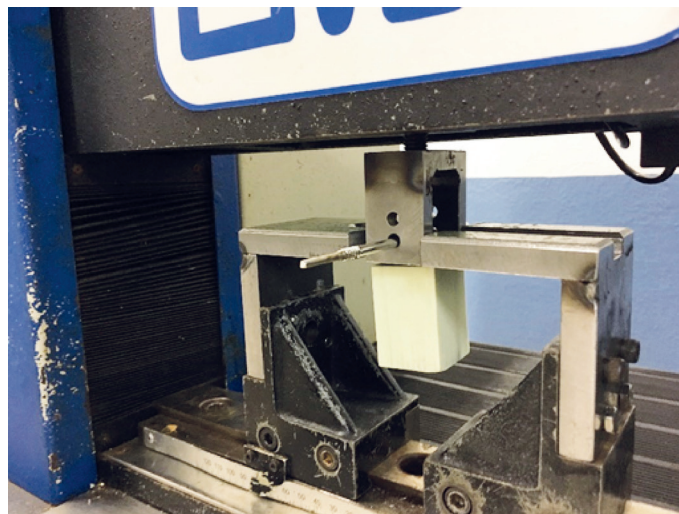
Figure 2. Polyurethane block individually mounted with screw for the application of pure axial load to measure pullout strength.
