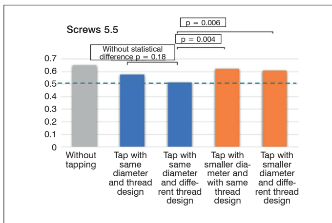
Figure 3. Mean insertion torque of the 5.5 mm screws with lines indicating p-values less than the adopted significance level ( p < 0.5 ) showing evidence of difference between the groups observed. Groups: 1 – without tapping, 2 – tapping with tap of diameter less than that of the screw and with the same thread design, 3 – tapping with tap of diameter less than the outer diameter of the screw with a different thread design, 4 – tapping with tap of the same outer diameter as the screw and the same thread design, and 5 – tapping with tap of the same outer diameter as the screw and a different thread design.
