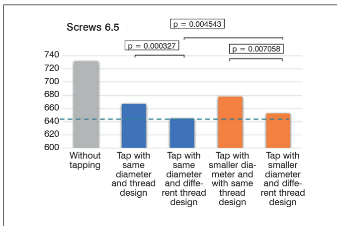
Figure 6. Mean pullout strength of the 6.5 mm screws with lines indicating p-values less than the adopted significance level ( p < 0.5 ) showing evidence of difference between the groups observed. Groups: 1 – without tapping, 2 – tapping with tap of diameter less than that of the screw and with the same thread design, 3 – tapping with tap of diameter less than the outer diameter of the screw with a different thread design, 4 – tapping with tap of the same outer diameter as the screw and the same thread design, and 5 – tapping with tap of the same outer diameter as the screw and a different thread design.
